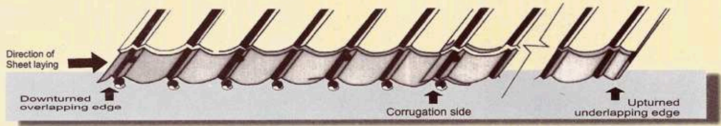
Location of Fasteners and Sheet Laying Procedure A = Depending on the length of the top tile Fastened to supports through the crest of the corrugations
