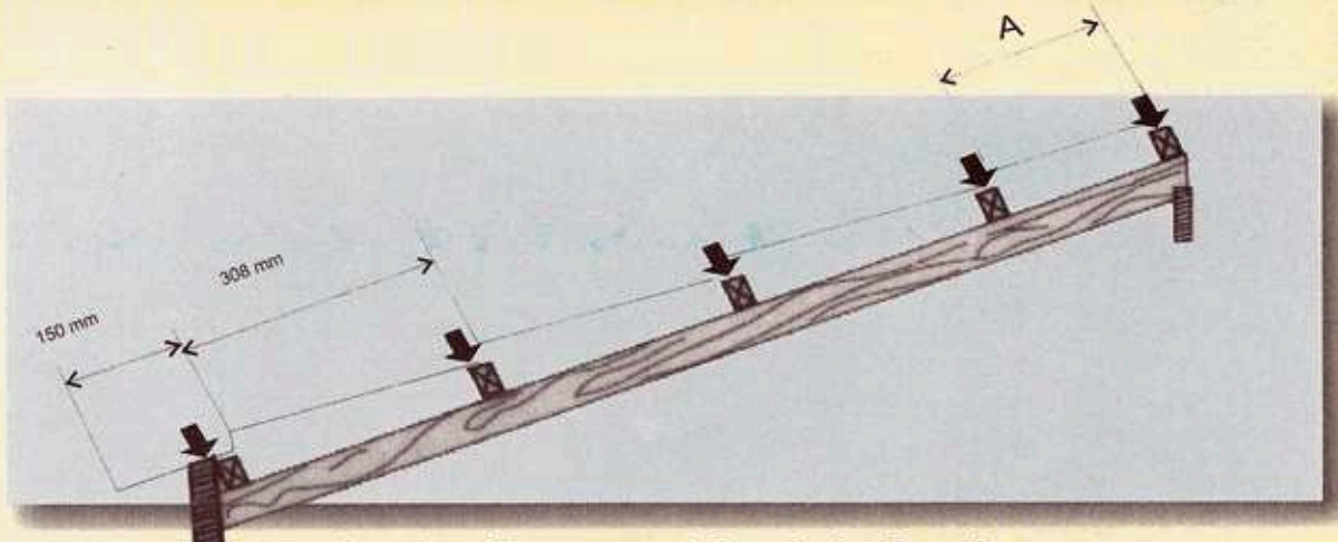
Location of Fasteners and Sheet Laying Procedure A = Depending on the length of the top tile Fastened to supports through the crest of the corrugations
